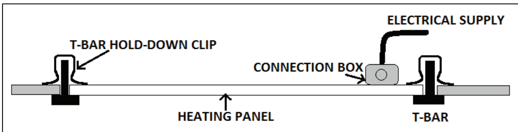
FIGURE 2 – T-Bar Mounting
