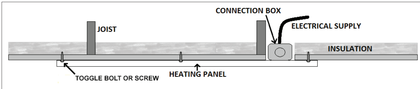
FIGURE 1 – Surface Mounting
