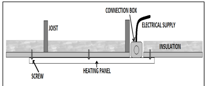
Figure 1 – Surface Mounting
